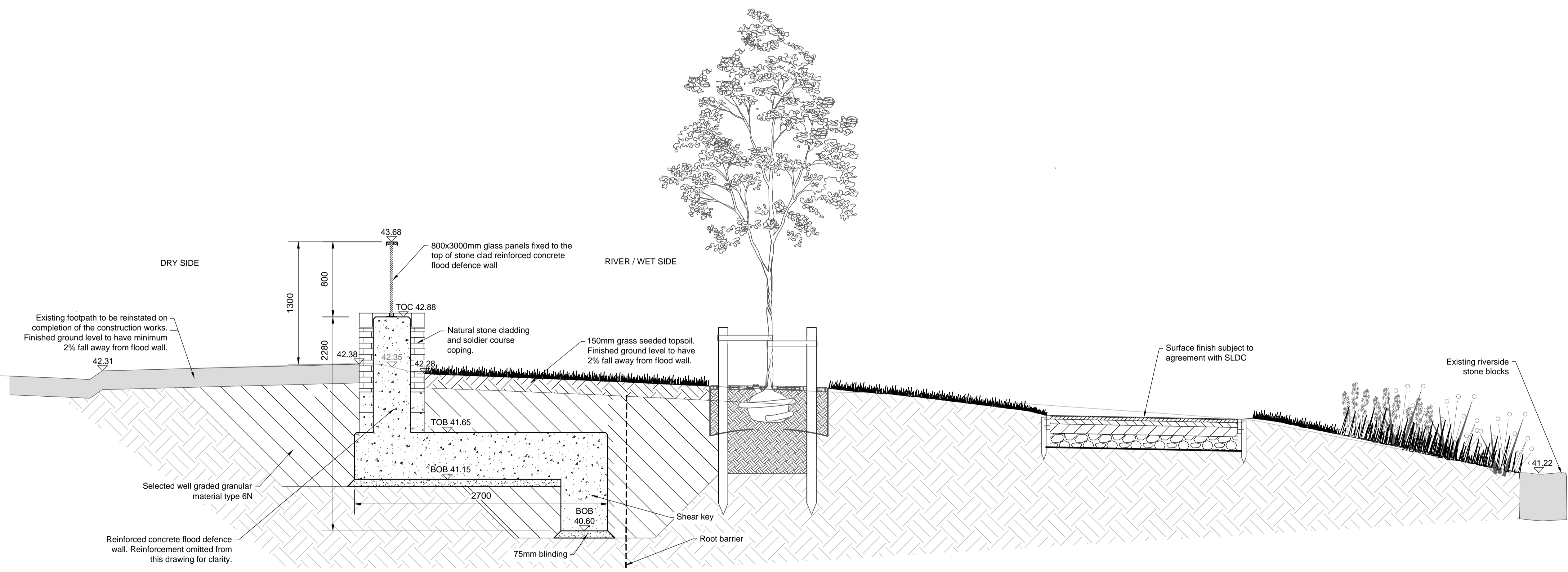
SECTION G-G SCALE 1:25 AT A1, 1:50 AT A3
