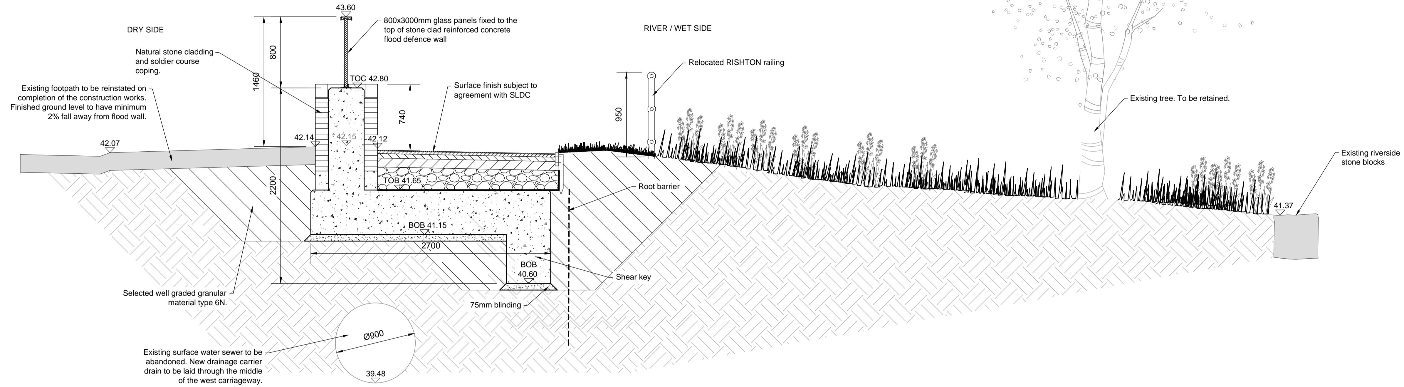
SECTION H-H SCALE 1:25 AT A1, 1:50 AT A3
