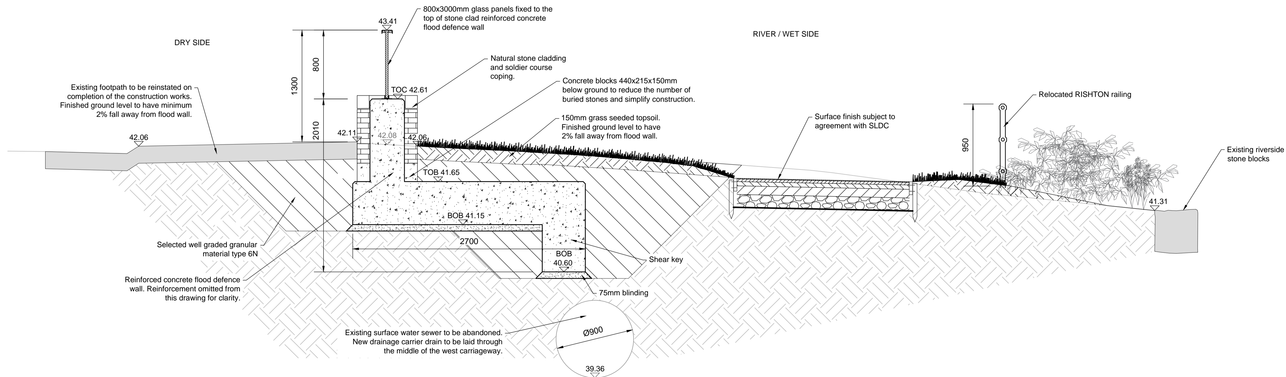
SECTION I-I SCALE 1:25 AT A1, 1:50 AT A3
