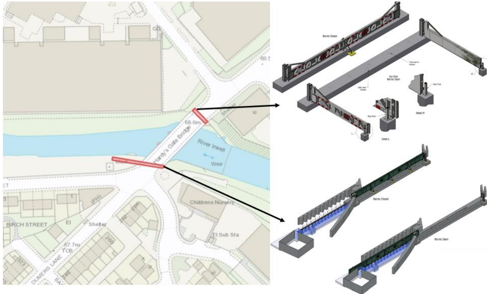
Figure 1: Map of gate locations and 3D renderings of north and south flood gates.
